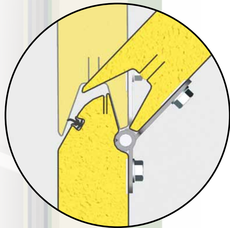
Articulations anti-pince doigts
